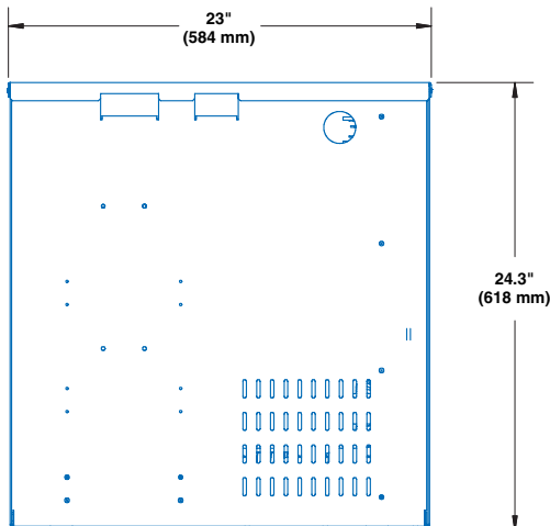
CABINET BACK
